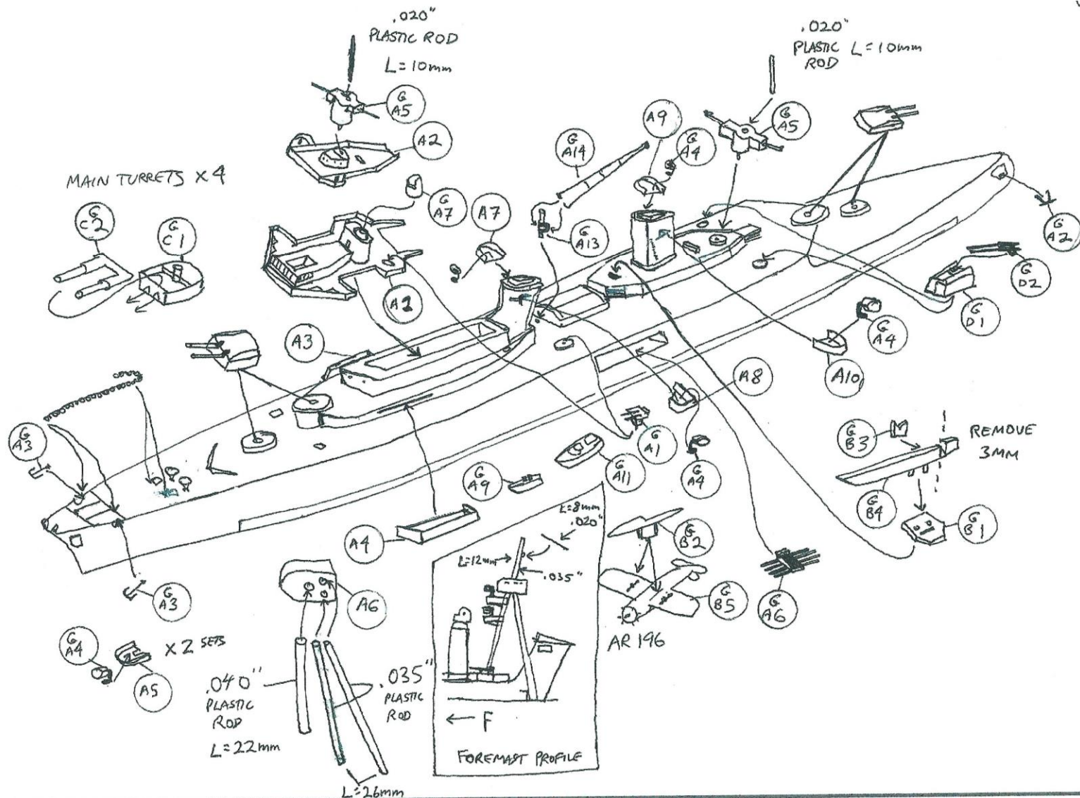
KREUZER M Kit. Scan of instruction sheet from our old resin kit, but most parts are the same. Some parts no longer included, such as Arado 196 aircraft. Also, anchor chain and plastic rod for masts not included.
